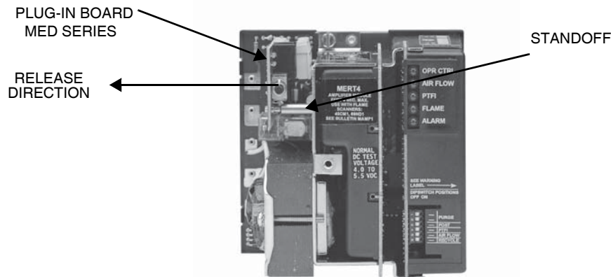
FIGURE 1. PLUG-IN BOARD LOCATION AND INSTALLATION
